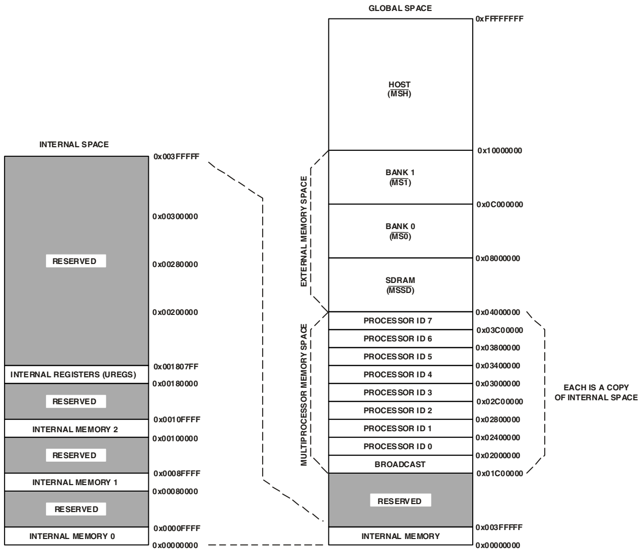
Figure 3. Memory Map
